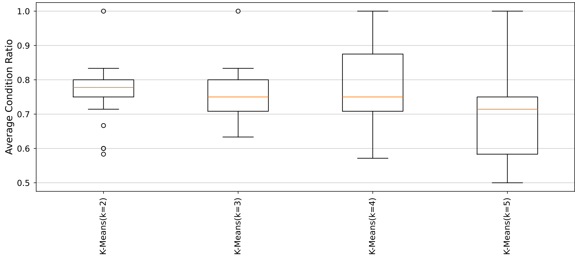
YARA Rules Average Condition Ratio Distribution (Cluster44_Size5 dataset)
